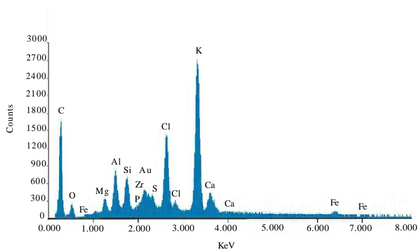
Fig. 2: EDX spectrum of tassel powder before use
