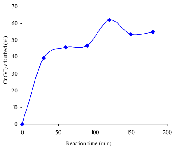
Fig. 7: Effect of contact time on Cr (VI) adsorption
