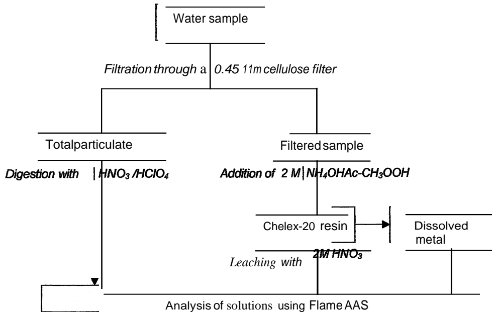
Figure 2. Scheme for the classification of metal species in the rivers in Thohoyandou.
