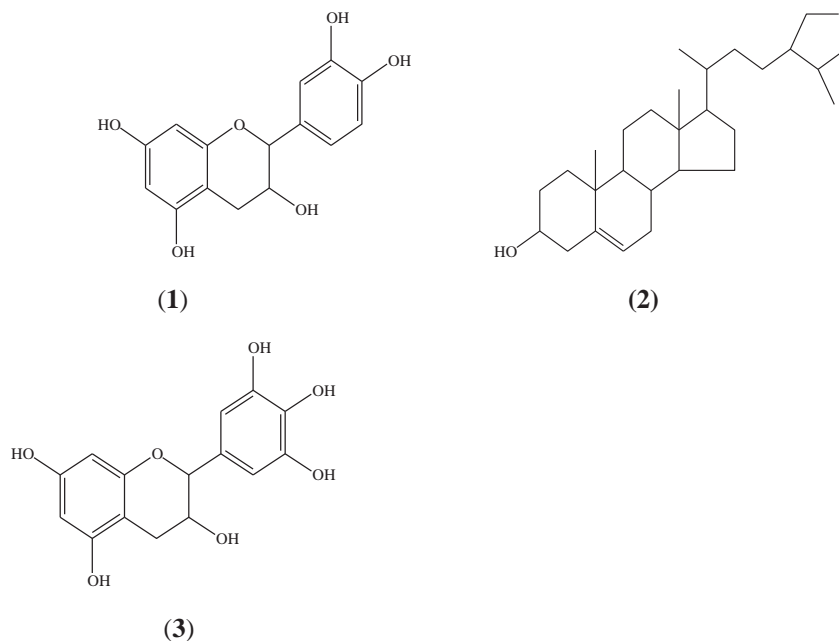
Fig. 1. Chemical structures of compounds isolated from the ethyl acetate extract of the leaves of A. karroo , (1) epicatechin; (2) β-sitosterol; (3) epigallocatechin.
