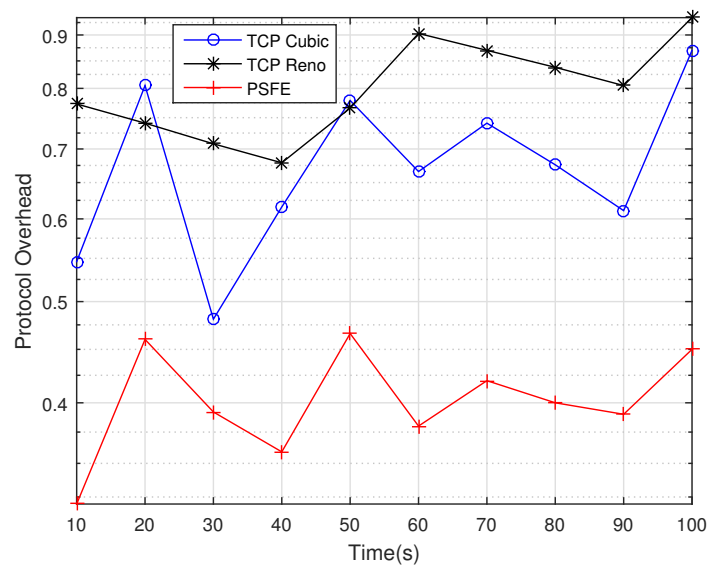
Figure 9. Comparisons of protocol overhead for packet-forwarding transmission.
