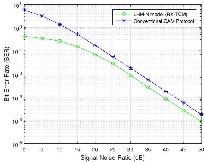
Figure 6. Comparative analysis of BER for LHM-N and the conventional QAM protocol.
