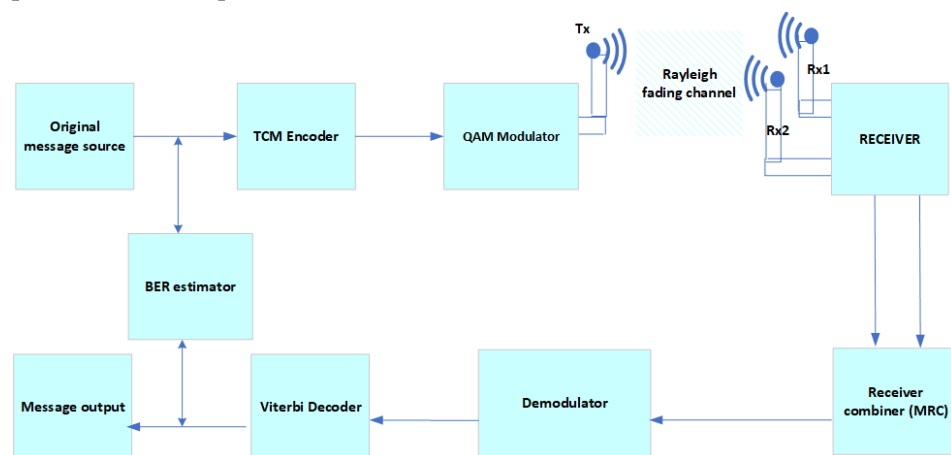
Figure 4. RX-TCM system model.png.
