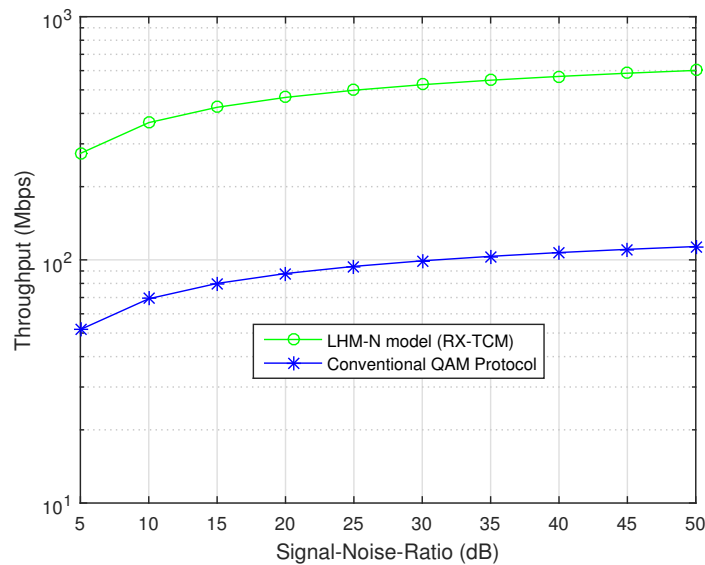
Figure 7. Comparative analysis of the throughput for LHM-N and the conventional QAM protocol.
