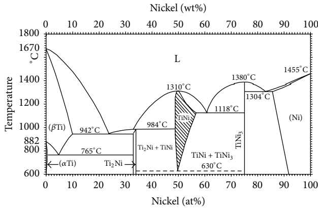
FIGURE 1: Equilibrium Ni-Ti phase diagram [20].
