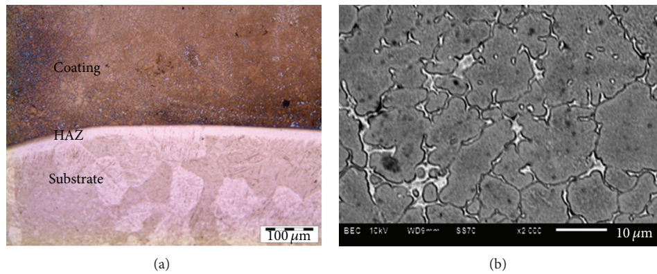
FIGURE 2: Micrographs of the laser deposited Ti50Ni50 coating; (a) optical image showing the interface of the coating and substrate; (b) SEM image of the coating.
