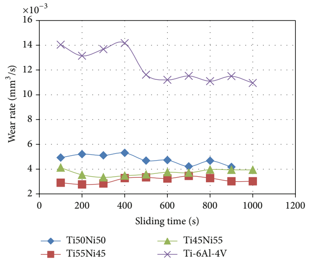
FIGURE 13: Wear rate analysis of laser deposited coating.
