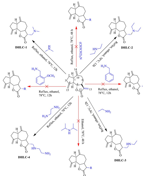
Scheme 2. Amination of C-13 double bond of dehydrocostus lactone.
