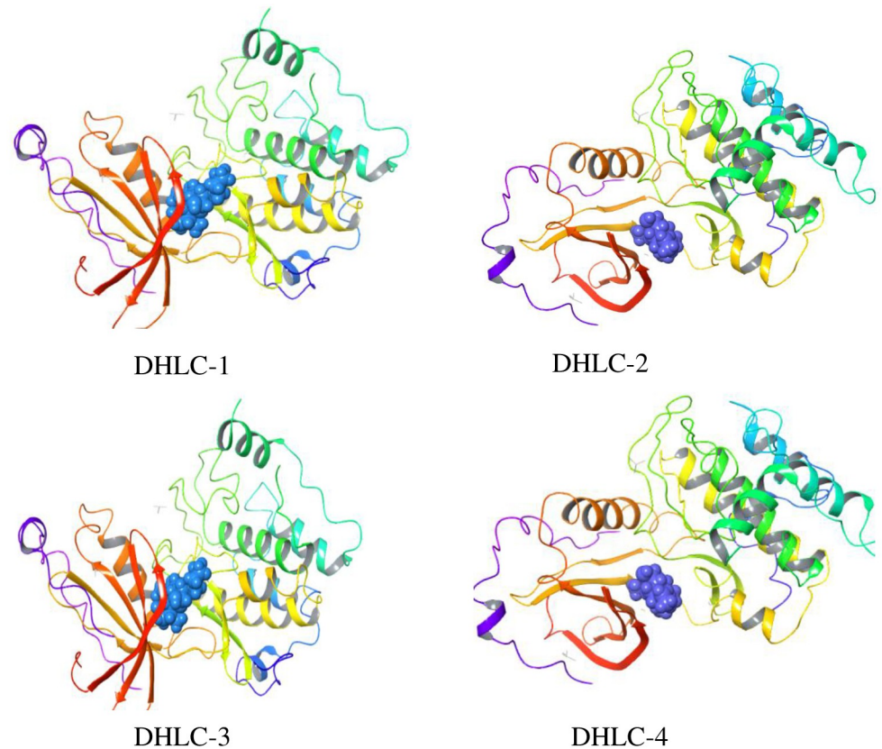
Fig 5. Best binding poses of 13-amino derivatives (DHLC-1-4) with 1ZRZ.
