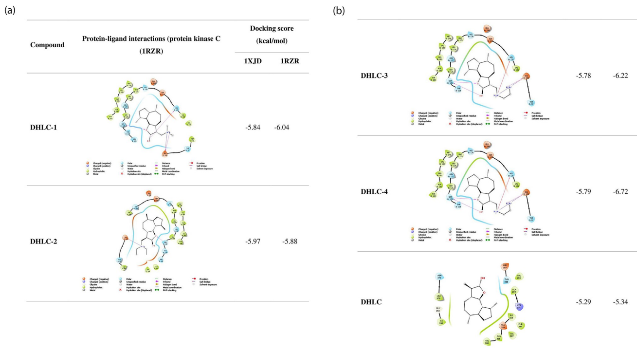
Fig 4. Molecular docking affinities of 13-amino derivatives of dehydrocostus lactone using protein kinase C (1RZR) and PKC theta (1XJD) enzymes.
