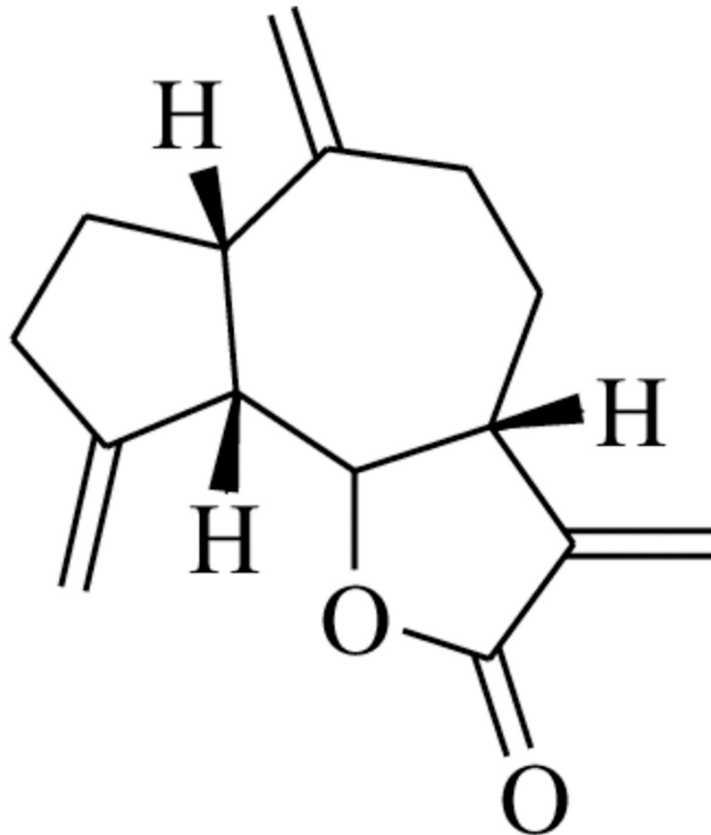
Fig 1. Structure of dehydrocostus lactone (DHLC).
