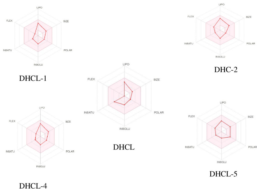
Fig 3. Bioavailability radar of the cytotoxic compounds. Note: The pink region indicates the optimal range for the properties predicted (size: Molecular weight between 140 and 400 g/mol, polarity: TPSA between 19 and 130 Å 2 , lipophilicity: XLOGP3 usually between -0.69 and + 4.9, saturation: fraction of carbons in the sp 3 hybridization not less than 0.25, solubility: log S not higher than 6, and flexibility: no more than 9 rotatable bonds [24].
