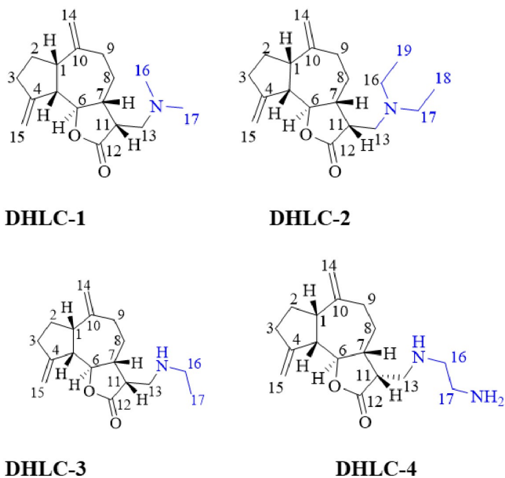
Fig 2. Structures of synthesized derivatives of dehydrocostus lactone.
